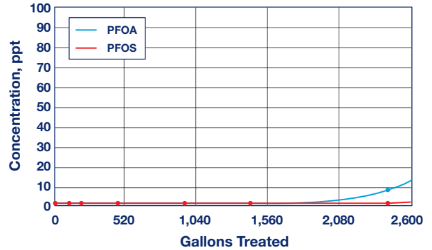
Filter Performance, AF-10-3612-BB for PFOS, PFOA Removal
