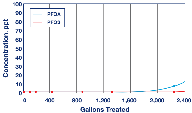
Filter Performance, AF-20-3612 for PFOS, PFOA Removal
