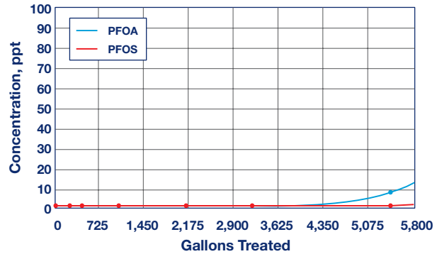
Filter Performance, AF-20-3612-BB for PFOS, PFOA Removal
