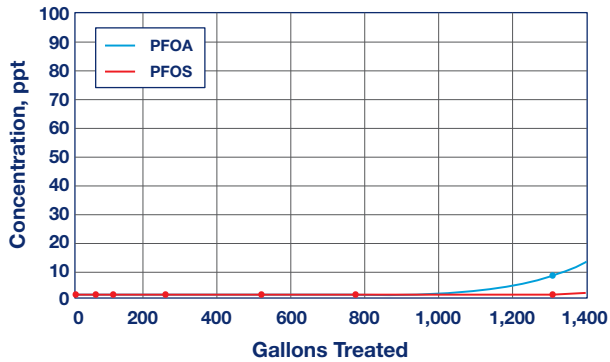
Filter Performance, AF-10-3612 for PFOS, PFOA Removal
