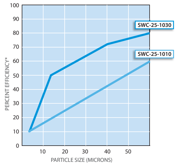
SWC Series Sediment Cartridges
